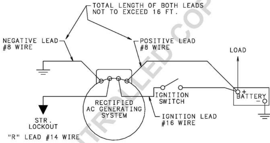
EXTERNAL WIRING DIAGRAM
