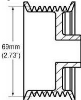
APS Part# F869 8 groove 69mm
