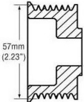
APS Part# G757 7 Groove 57mm
