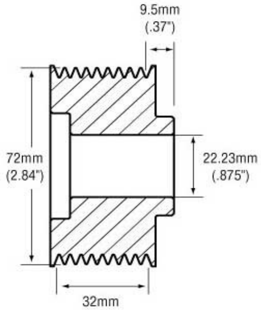
APS Part Number L9-72S9.5
