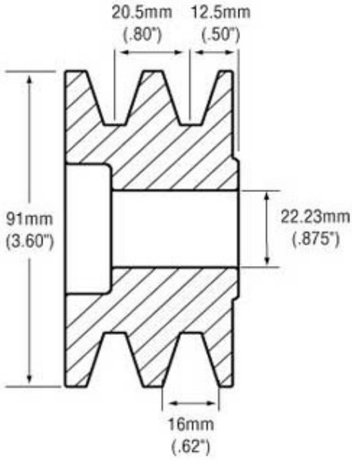
APS Part Number L2-91V12.5
