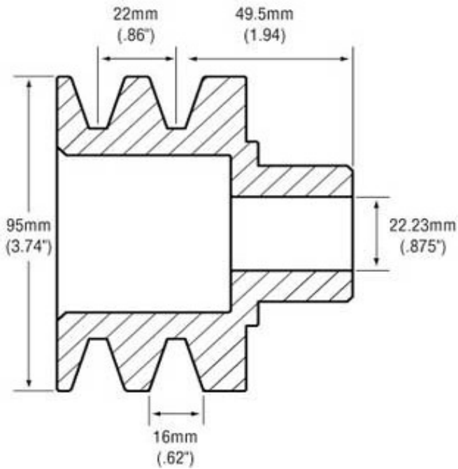
APS Part Number L2-95V49.5
