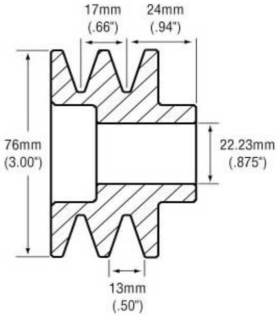
APS Part Number L2-76V24
