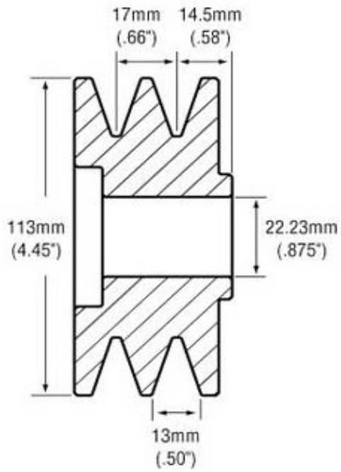
APS Part Number L2-113V14.5
