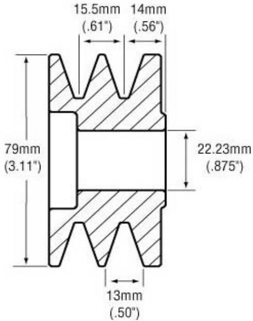
APS Part Number L2-79V14
