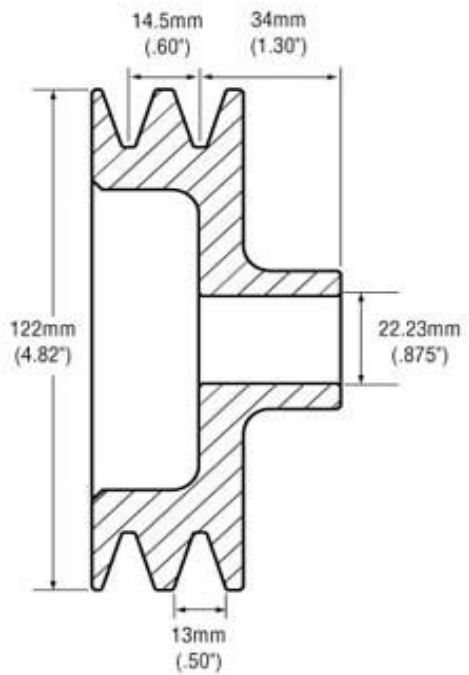
APS Part Number L2-122V34
