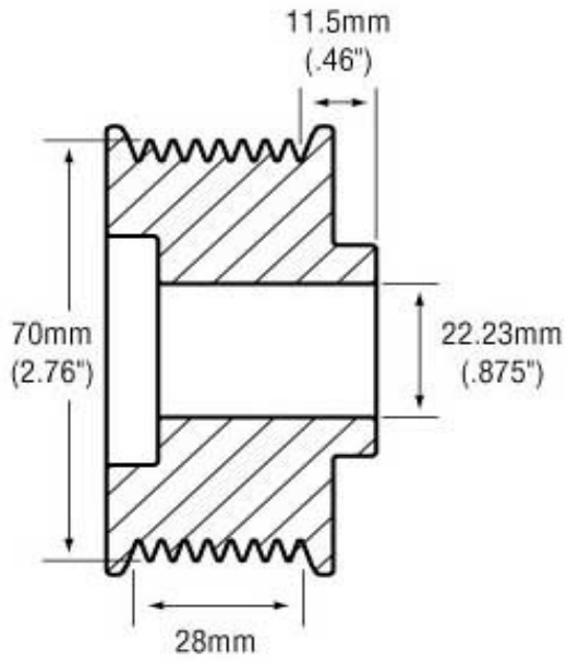
APS Part Number L8-70S11.5
