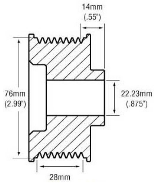
APS Part Number L8-76S14
