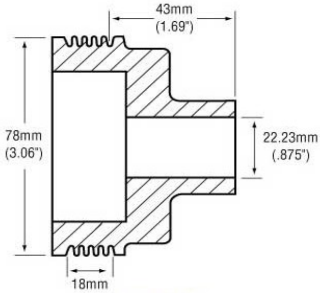
APS Part Number L5-78S43
