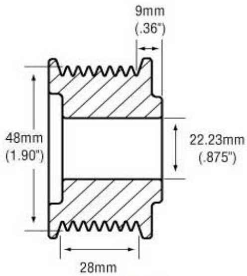
APS Part Number L8-48S9
