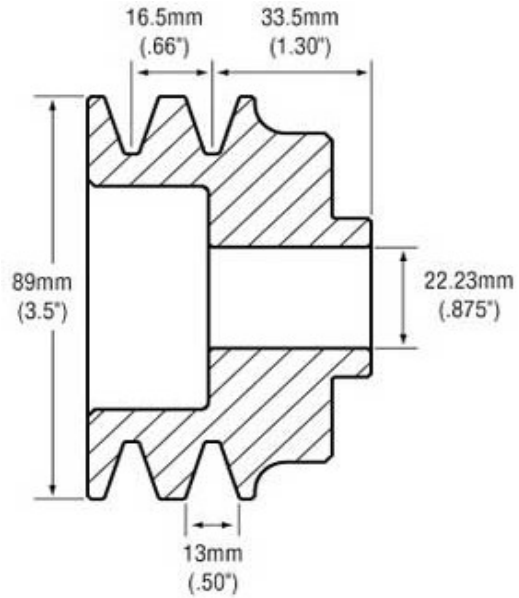
APS Part Number L2-89V33.5
