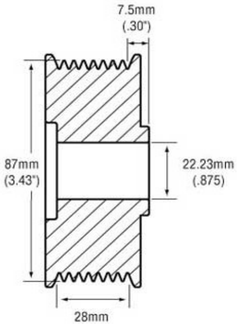
APS Part Number L8-87S7.5
