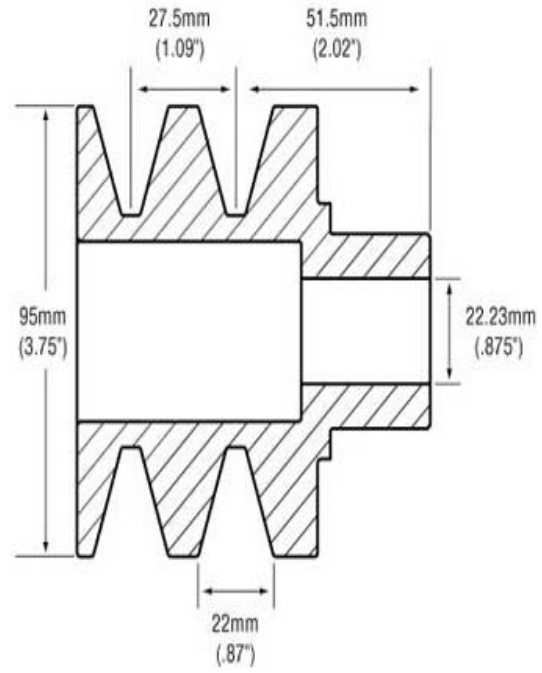
APS Part Number L2-95V51.5
