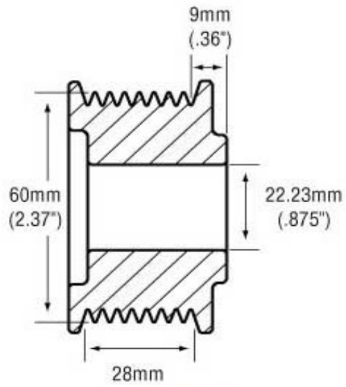
APS Part Number L8-60S9
