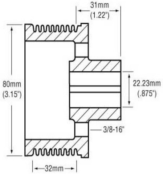
APS Part Number L9-80S31
