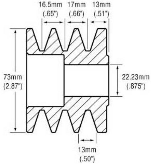
APS Part Number L3-73V13
