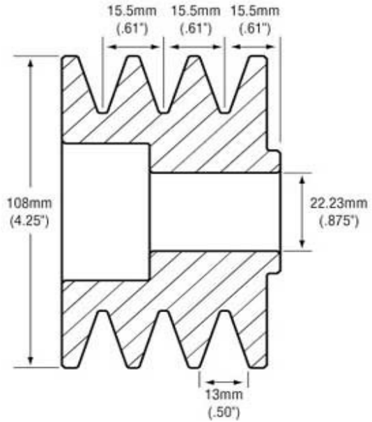
APS Part Number L3-108V15.5
