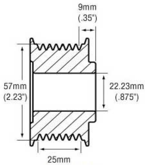
APS Part Number L7-57S9
